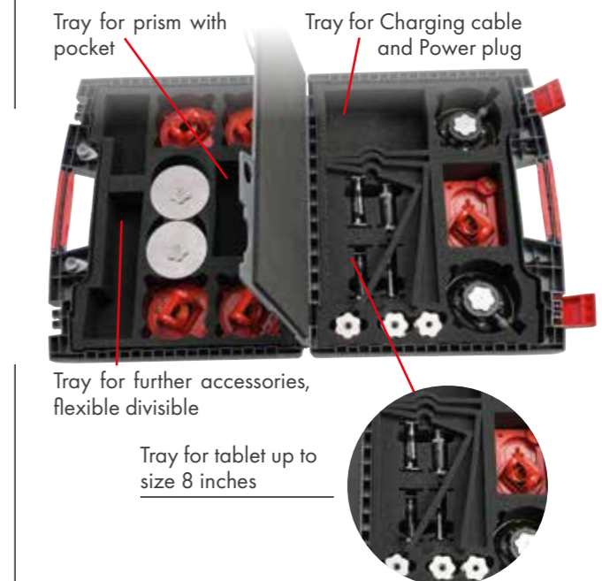
Fig. KS1-390M+C/S-2 Metrics: W 500 mm x H 420 mm x D 225 mm Weight (without tablet an additional accessories): 7.8 kg
