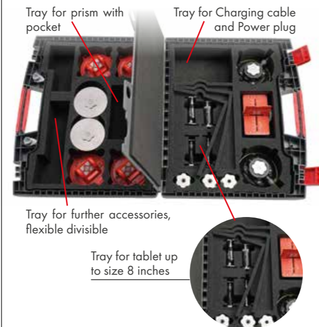
Fig. KS1-193M+-2 Metrics: W 500 mm x H 420 mm x D 225 mm Weight (without tablet an additional accessories): 7.8 kg
